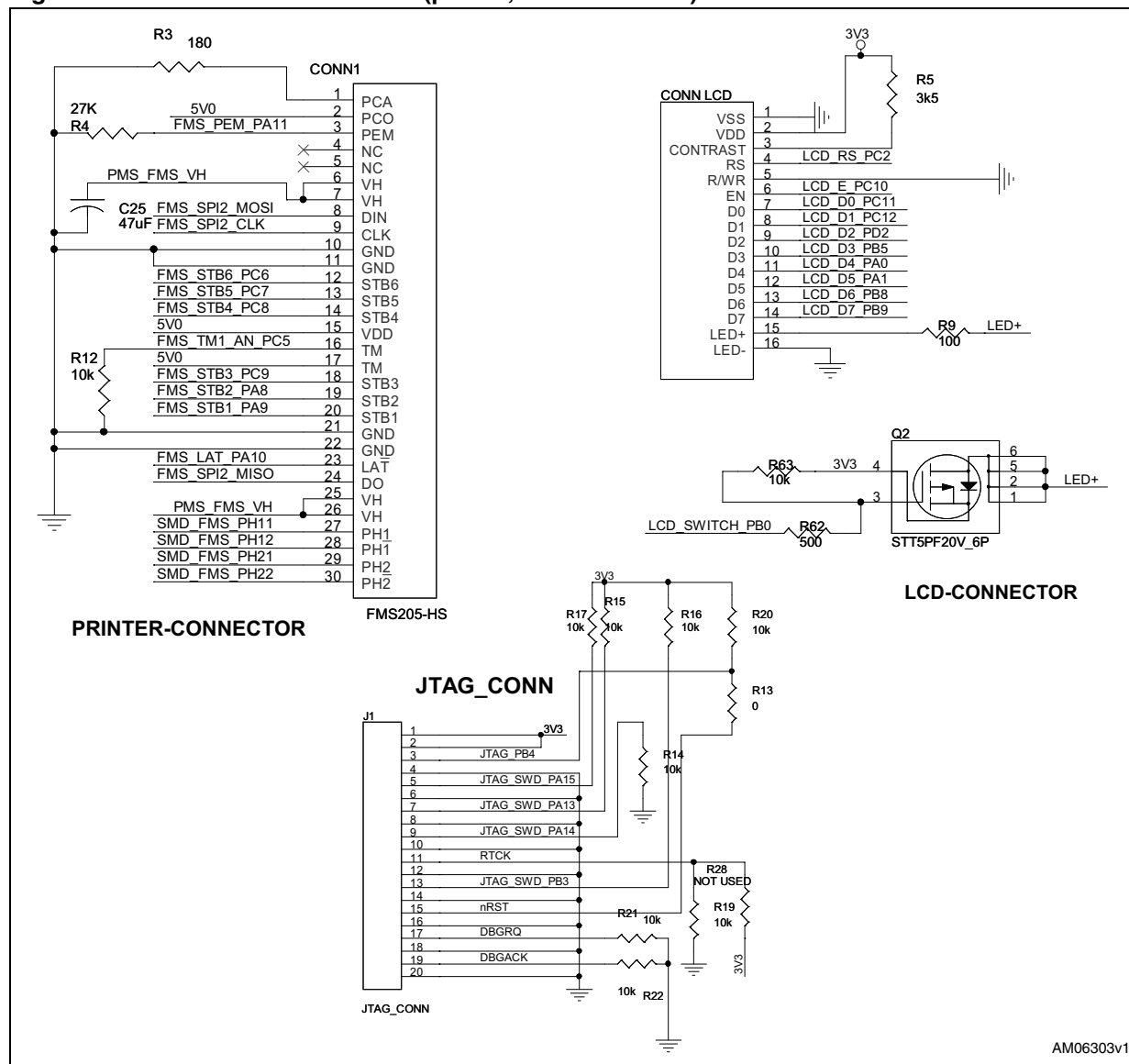
Figure 17. Schematic: connectors (printer, LCD and JTAG)
